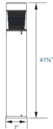
Flat Top Bollards
