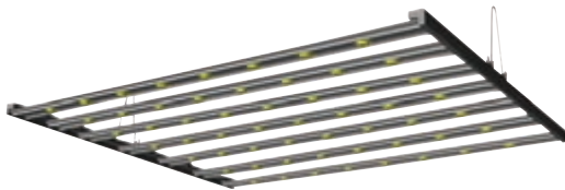
GL73C3 COB: 240w Color Spectrum: Red: 77.1% Blue: 22.6% Green: .3% Nanometer Ranges: Red: 600-699 Blue: 400-499 Green: 500-599
